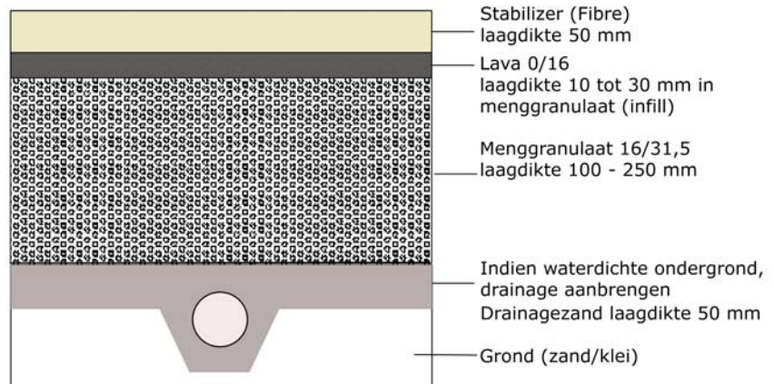
Doorsnede Stabilizer / Stabilizer Fibre
